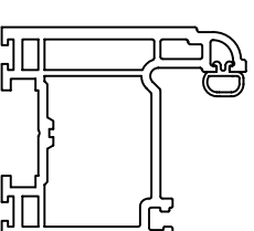
BOTTOM SASH
