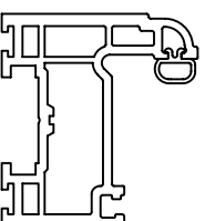
TOP SASH
