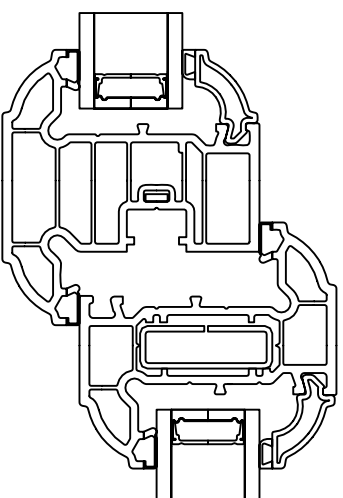
SASH / MULLION DETAIL
