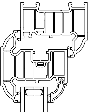
FRAME / SASH DETAIL
